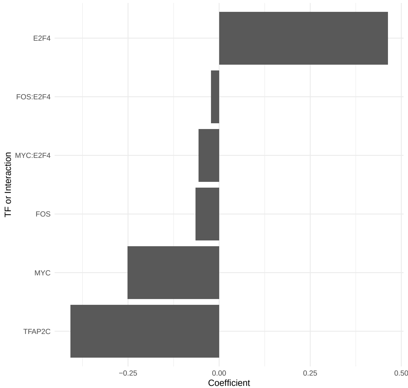
TF and TF:TF interactions predictive of ENSG00000007968.6
